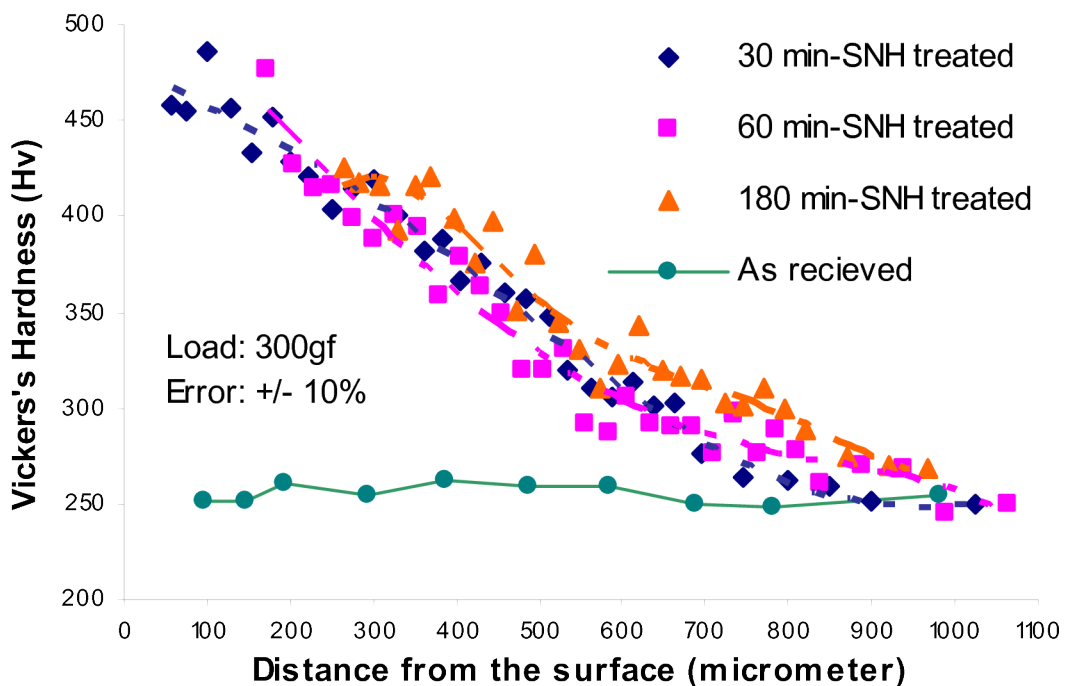
Figure 11. Hardness profile of the samples [80].
