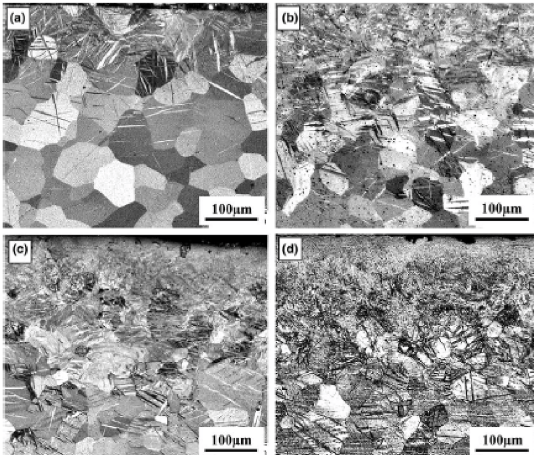
Figure 2: Typical cross-sectional optical micrographs close to the SMAT-treated surfaces under different treating conditions (annealed, commercially pure titanium specimens): (a) vibration amplitude 50%, treatment time 10s; (b) vibration amplitude 50%, treatment time 16s; (c) vibration amplitude 100%, treatment time 30s; (d) vibration amplitude 100%, treatment time 60s [57].
