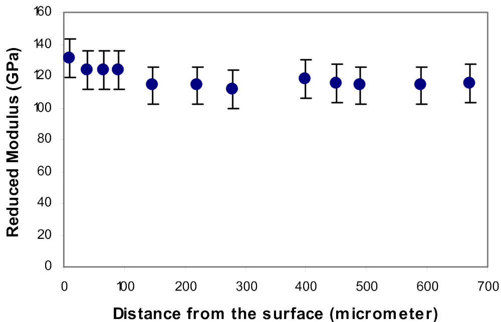
Figure 7: Reduced modulus versus the distance for the sample surface for a load P=10 \text{ mN} [88].
