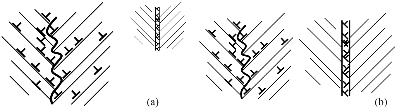
Figure 1: Arrangement of grain boundaries in nanostructured layers (a) the dislocation structure during SPD processing (b) the dislocation structure after SPD processing leading to formation of non-equilibrium grain boundaries.
