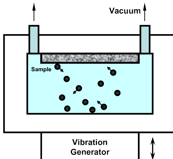
Figure 4: Sketch of SMAT.
