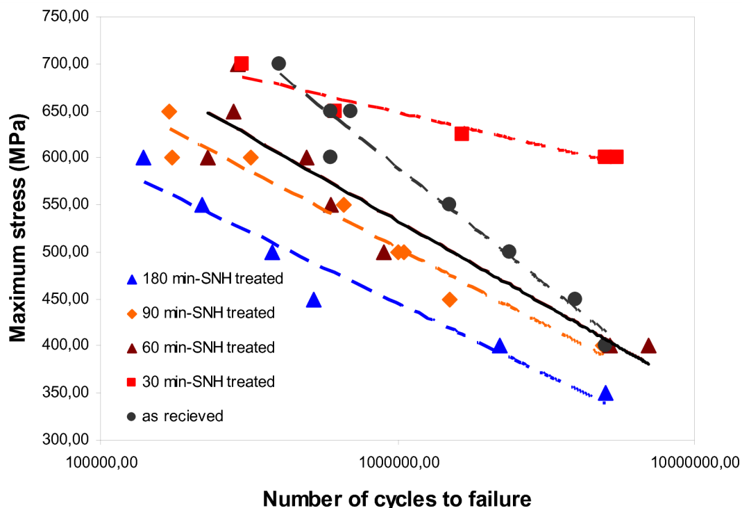
Figure 5. Fatigue behavior of SNH treated Ni-based C-2000 super alloy samples [80].
