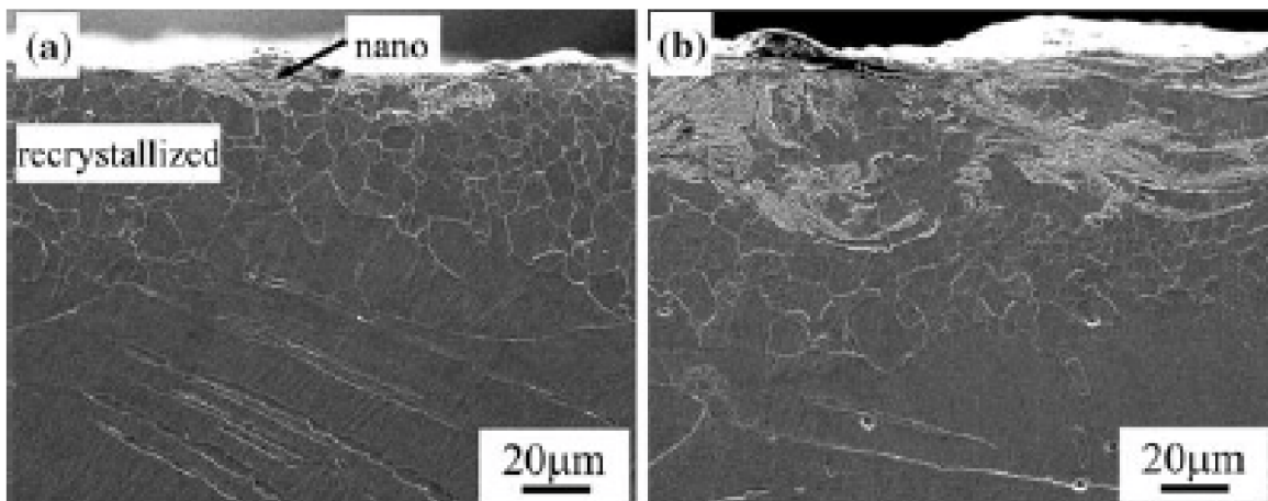
Figure 10: Microstructure of shot peened Fe-3.29Si after annealing at 873 K for 3.6 ks: (a) 3,000%, (b) 10,000% [19].
