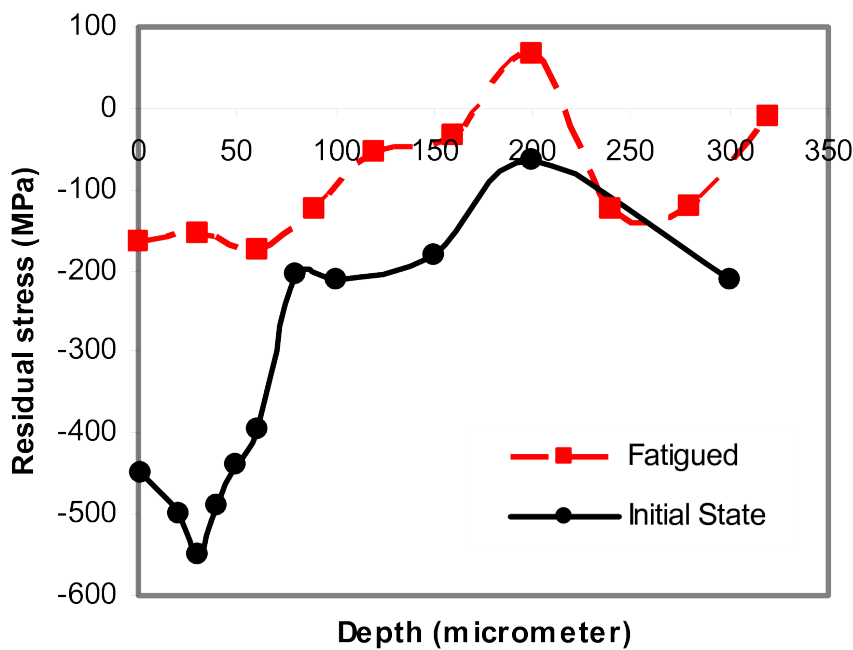
Figure 6. Residual stress depth profiles of shot peened (Almen intensity 0.175 mmA) AISI 304 before and after cyclic loading with \sigma_a = 320 \text{ MPa} after N_f/2 cycles [62].
