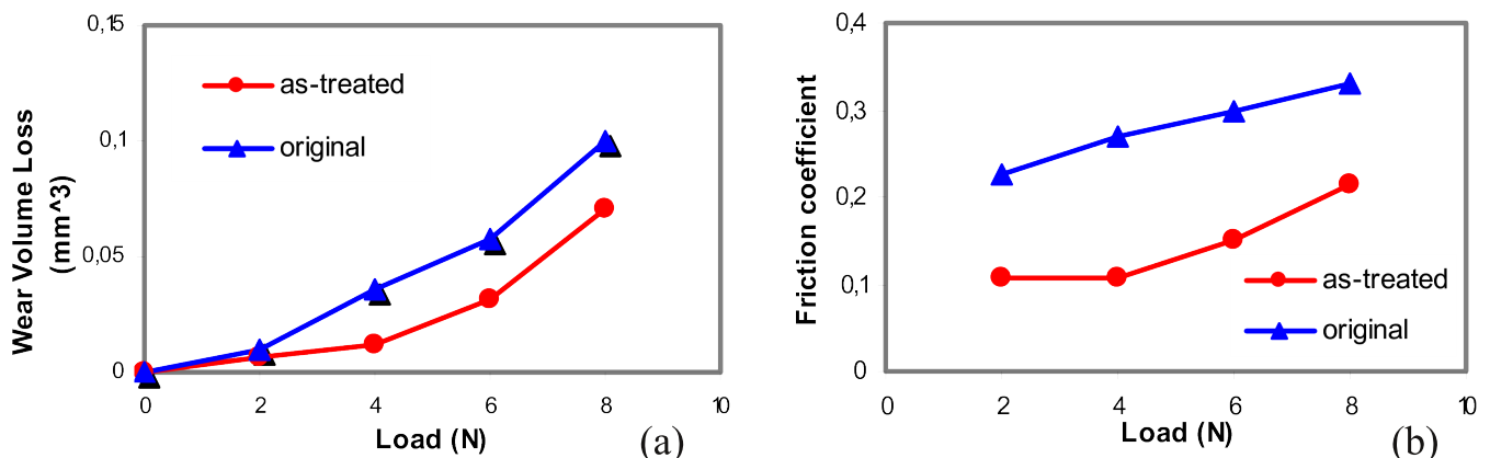
Figure 8: Variations of the wear volume loss with load (a) and variations of the coefficient of friction with load (b) for the SMAT and the original low-carbon steel samples [73].
