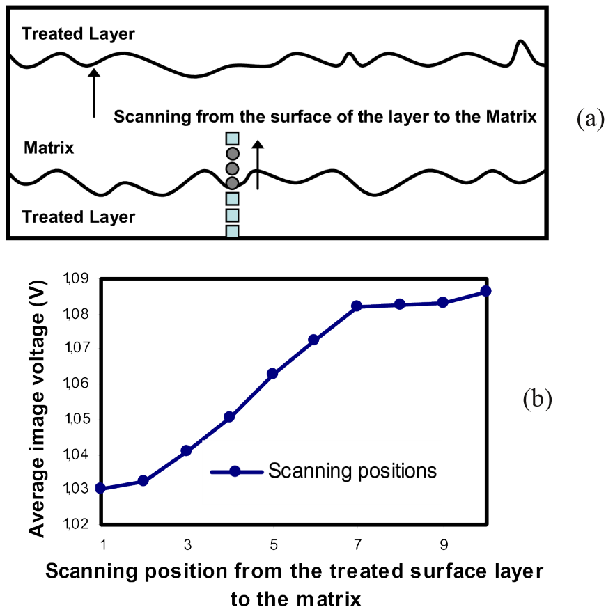
Figure 12: (a) Schematic diagram of the scanning positions from the surface layer to the matrix on the cross-sectional surface. (b) Variation in average image voltage while scanning from the treated surface layer to the matrix as indicated in (a) [97].
