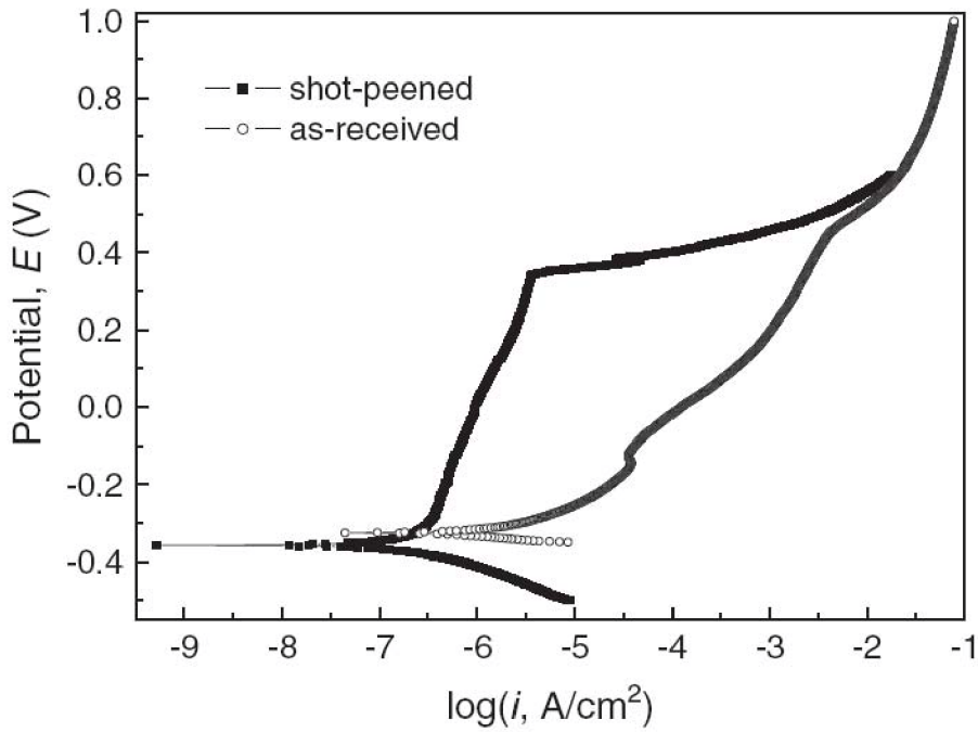
Figure 9: Potentiodynamic polarization curves of shot-peened and as-received samples of 1Cr18Ni9Ti stainless steel obtained in 3.5% NaCl solution [55].
