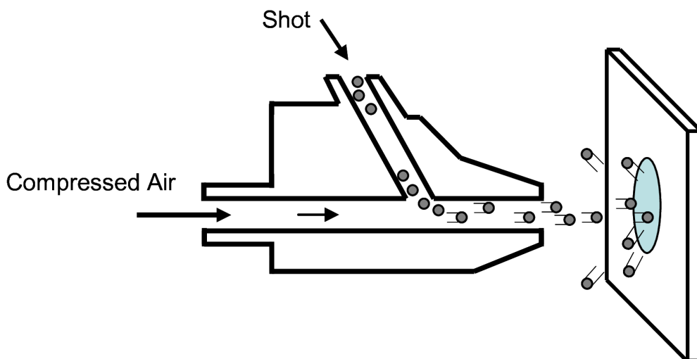
Figure 3: Schematic illustration showing the equipment of ABSP.
