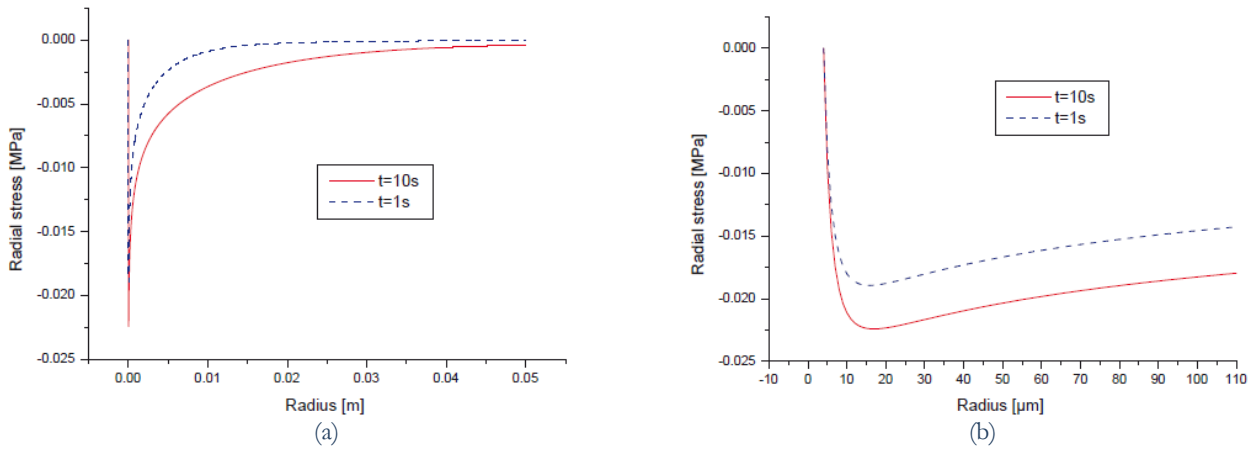
Figure 2: The distribution of the radial normal stress for various times for a unit heat source q = 1 \text{ Wm}^{-1} and r_R = 4 \text{ μm} ; a) general view, b) enlargement near the reverse cyclic plastic zone.
