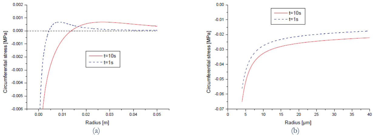
Figure 3: The circumferential stress distribution at various times for a unit heat source q = 1 \text{ Wm}^{-1} and r_R = 4 \text{ μm} ; a) general view, b) enlargement near the reverse cyclic plastic zone.
