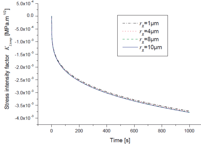
Figure 4: The stress intensity factor K_{I,temp} due to thermal stresses versus time for different radius of the reverse cyclic plastic zone.
