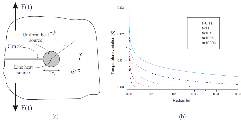
Figure 1: a) Schematic of the thermomechanical problem of a semi-infinite crack in an infinite plate under cyclic tension (mode I) caused by a remotely mechanical loading F(t) , and b) The temperature variation field near the crack tip for q = 1 \text{ W m}^{-1} .
