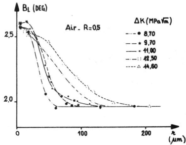
Figure 3 Distribution of the residual stresses and peak breadths below the surface for test at R = 0.5 in air
