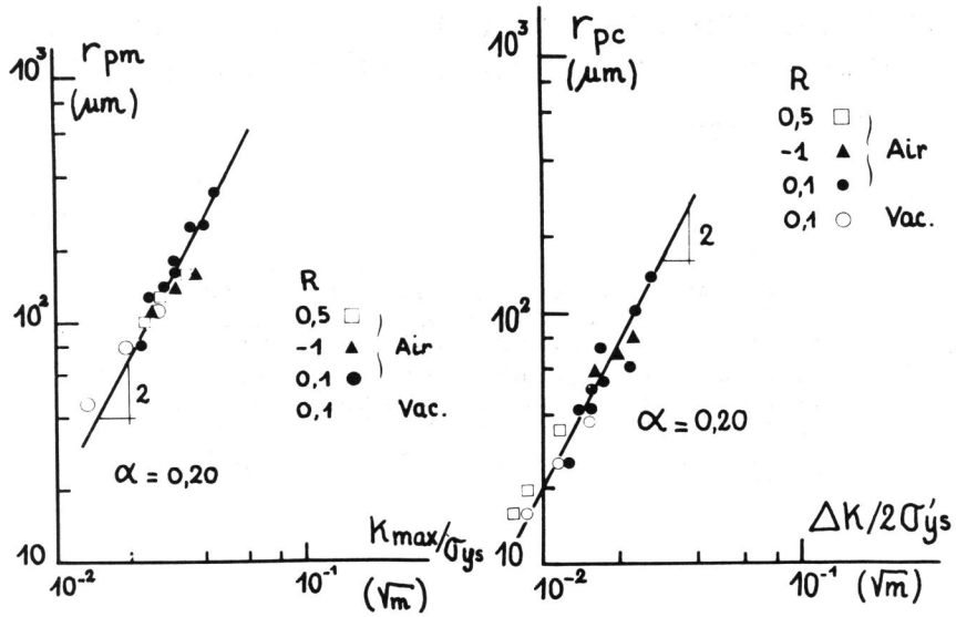
Figure 9 Relationship between the cyclic plastic zone size and \Delta K/2\sigma'_{ys}
