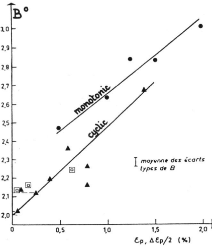
Figure 2 Relationship between the peak breadth B and the plastic strain
