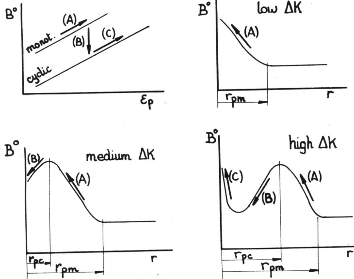
Figure 7 Schematic representation of peak breadth evolution in-depth for different levels of \Delta K
