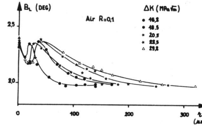
Figure 4 Distribution of the residual stresses and peak breadths below the surface for at R = 0.1 in air
