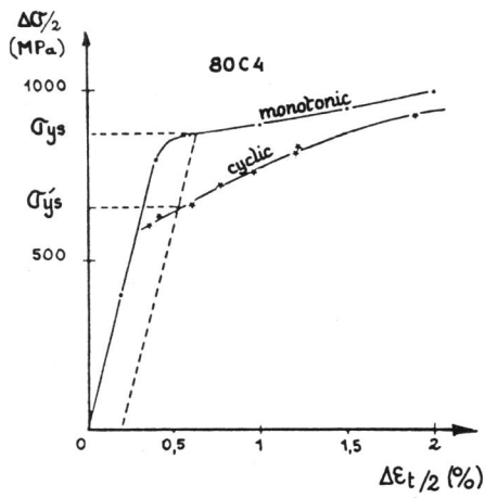
Figure 1 Monotonic and cyclic stress and strain behaviour of the 80C4 steel
