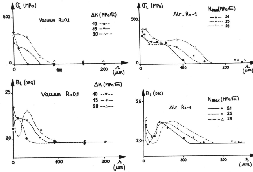
Figure 5 Distribution of the residual stresses and peak breadths below the surface for test at R = 0.1 in vacuum
