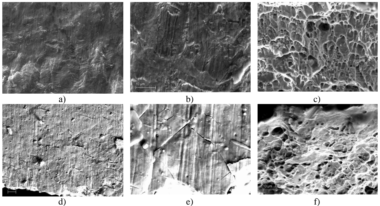
Fig. 3. SEM micrographs for the area of fatigue crack growth found at the flat face (a, b, d, e) and fracture surface of specimens (c, f), failed at cyclic tension tests; (a-c) specimens without treatment; d-f) with nanostructured surface layer; (a, b, d, e) axis of loading oriented vertically
