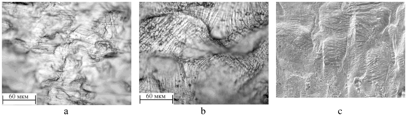
Fig. 2. Surface images of failed specimens at static tensile tests: a) specimen without treatment; b), c) after nanostructuring surface; a), b) optical images, axis of loading is oriented horizontally; c) SEM-microphotographs, axis of loading is oriented vertically
