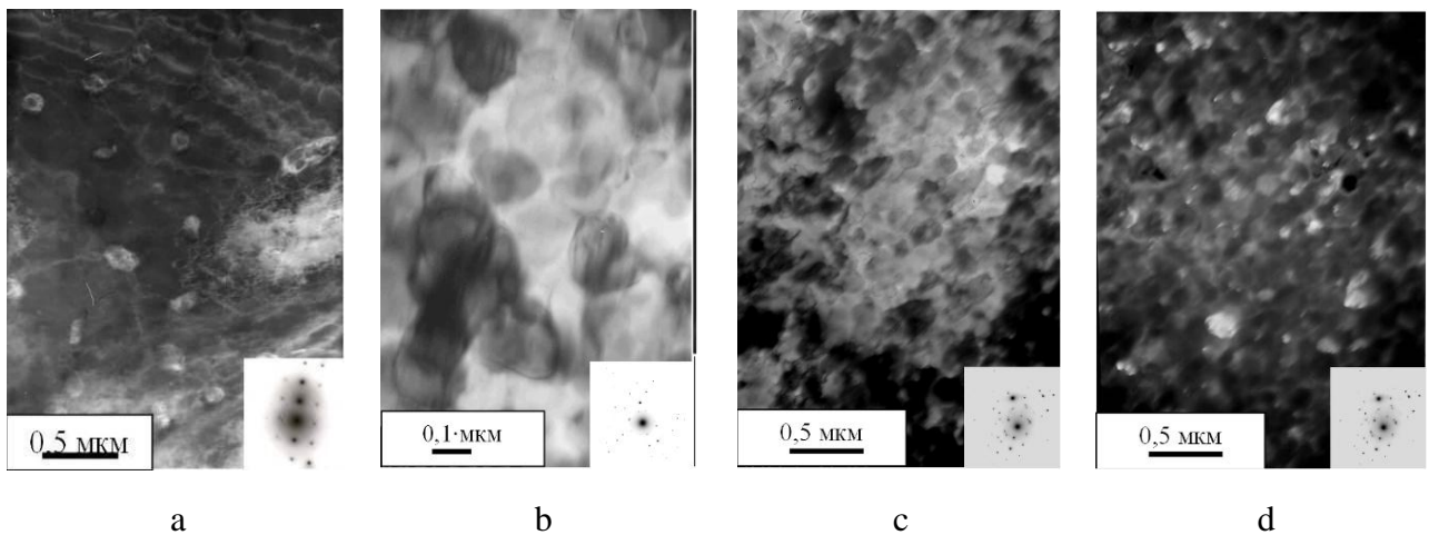
Fig. 1. SEM images of the structure of subsurface layer of 12Cr1MoV steel: a) initial state; b), c), d) after nanostructuring; a), d) dark field; b), c) light field
