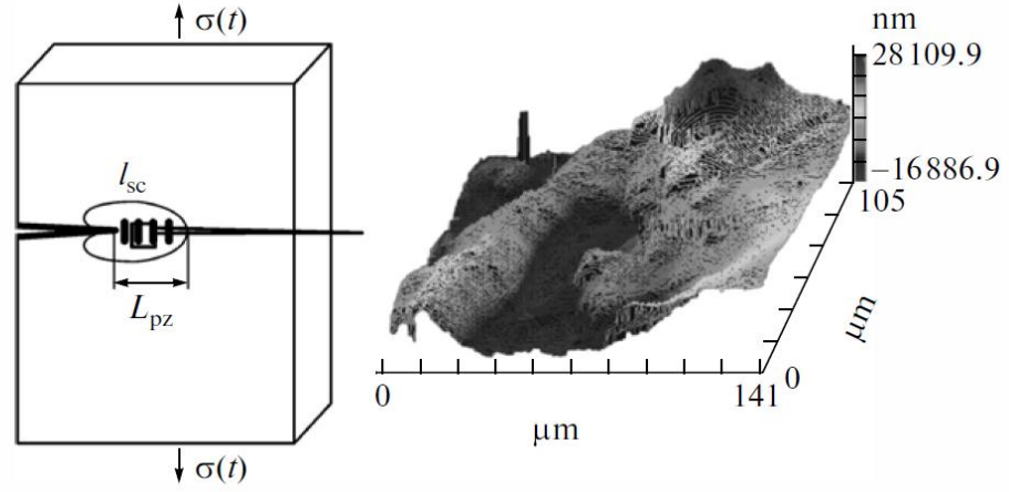
Fig.2. Schematic diagram showing a region at the crack tip and typical image of the surface relief.
