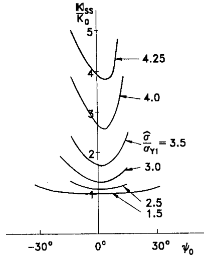
Figure 3: Steady–state interface toughness as a function of the local mixity measure \psi_0 , for \sigma_{Y1}/E_1 = 0.003 and \sigma_{Y2} \approx \infty , considering different values of \hat{\sigma}/\sigma_{Y1} , E_2/E_1 = 2 . (From [23]).
