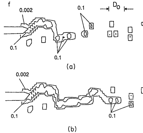
Figure 1: Crack growth indicated by contours of constant void volume fraction, f , for random distribution of larger particles. (a) t = 1.5 \mu\text{s} , \Delta a = 0.09 \text{ mm} ; (b) t = 1.6 \mu\text{s} , \Delta a = 0.27 \text{ mm} . (From [9]).
