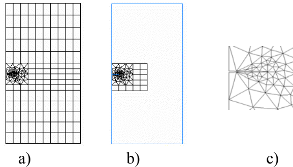
Figure 2: Typical mesh model: a) of the plate b) of the patch c) near the crack tip
