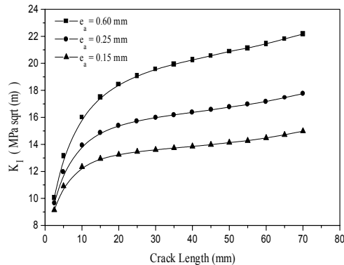
Figure 5: Effect of the adhesive thickness the mode I stress intensity factor variation ( G_a=500 Mpa, W_r = 75 mm, e_r=1.3 mm)
