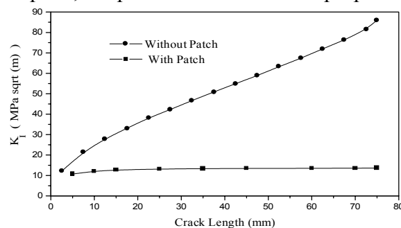
Figure 3: Comparison of the stress intensity factor between patched and unpatched cracks.
