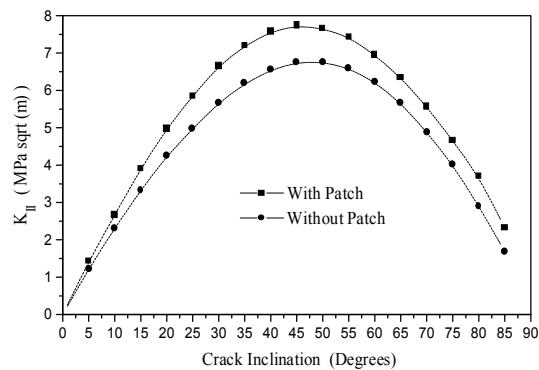
Figure 8: Comparison of the mode II stress intensity factor between patched and unpatched crack in mixed mode ( a = 25 mm).
