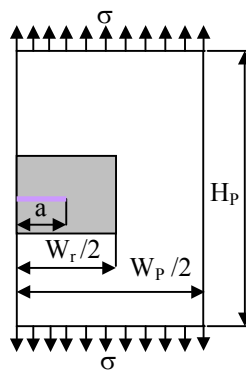
Figure 1: Geometrical model of the half of the patched structure in mode I.
