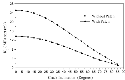
Figure 7: Comparison of the mode I stress intensity factor between patched and unpatched crack in mixed mode ( a = 25 mm).
