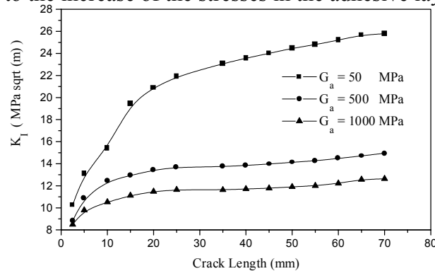
Figure 4: Effect of the adhesive shear modulus on the mode I stress intensity factor variation ( e_a=0.13 mm, W_r=75 mm, e_r=1.3 mm)
