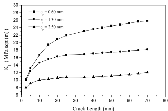
Figure 6: Effect of the patch thickness on the mode I stress intensity factor variation ( G_a= 500 Mpa, e_a=0.13 mm, W_r = 75 mm)
