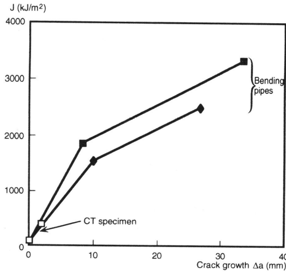
Figure 8 : Comparison of J-resistance curves of A42 carbon steel obtained with bending pipes and CT specimens.
