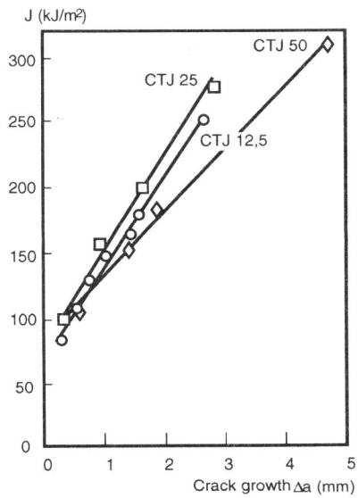
Figure 3 : Comparison of J-resistance curves of low upper shelf energy C-Mn steel obtained with 1/2T-, 1T- and 2T-CT specimen.
