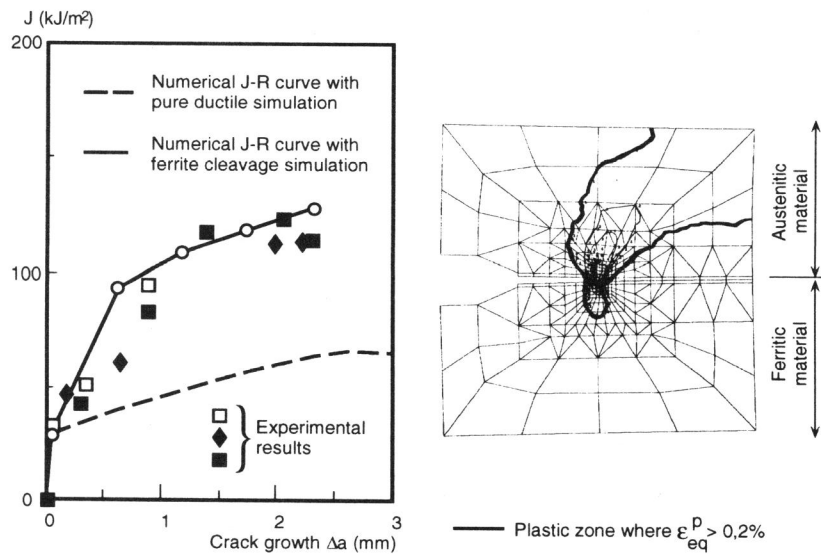
Figure 6 : Comparison of experimental and numerical J-resistance curves of aged duplex stainless steel.
