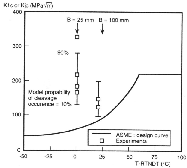
Figure 9 : Comparison of the experimental results and prediction of the toughness of A508 Cl 3 steel in the transition regime.
