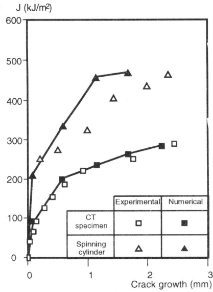
Figure 1 : Comparison of J-resistance curves derived from first spinning cylinder and CT-specimen tests.
