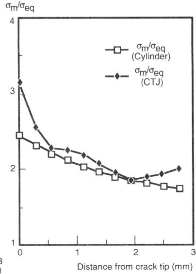
Figure 2 : Comparison of stress triaxiality at crack tip in the first spinning cylinder and CT-specimens.
