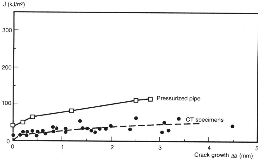
Figure 5 : Comparison of experimental J-resistance curves of aged duplex stainless steel obtained with burst test pipe and CT specimen.
