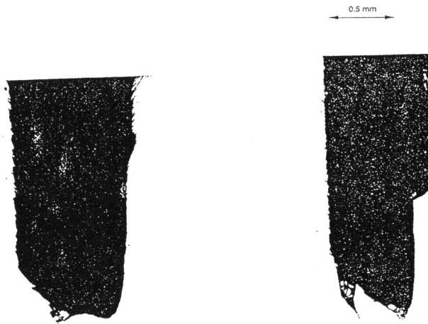
Fig 7 Crack tip profiles for Mixed Mode I/II loading a) Position 3 b) Position 4
