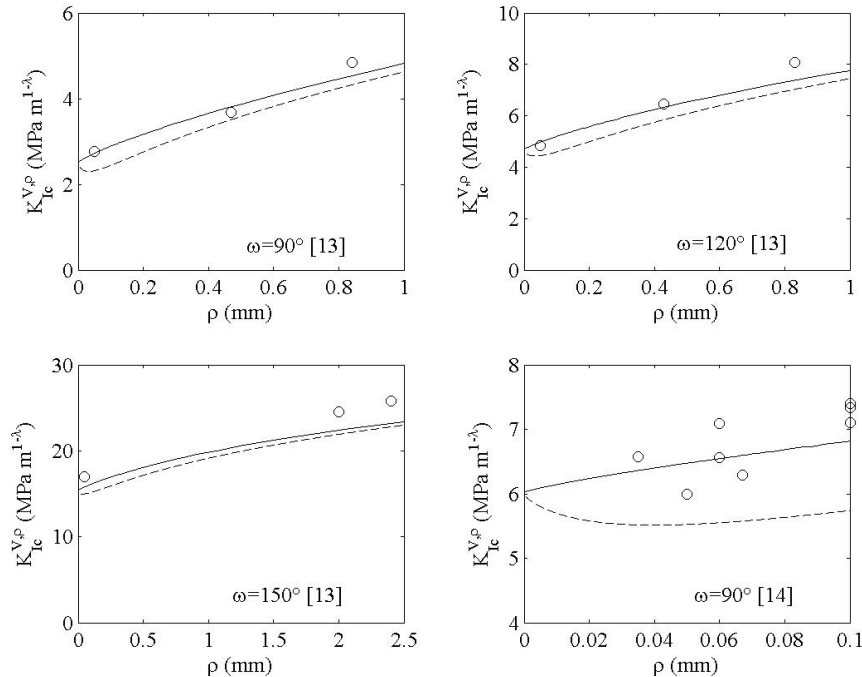
Figure 2: K_{Ic}^{V,\rho} vs. \rho experimental data (circle) and theoretical predictions according to the PS criterion (dashed line) and FFM.
