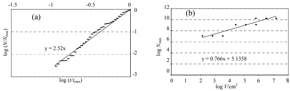
Figure 1: Space-time scaling in damage evolution.
