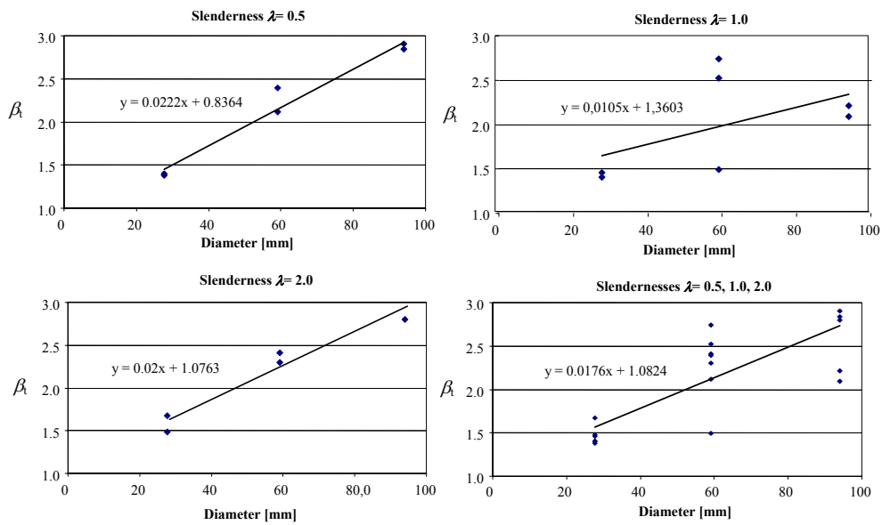
Figure 2: Life-time exponent \beta_l plotted vs. specimen diameter.
