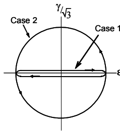
Figure 2. Strain paths employed.
