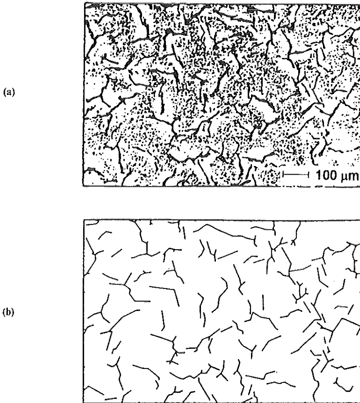
Fig 1 Crack pattern after 4500 load cycles: (a) observed via an optical microscope; (b) after digitizing.
