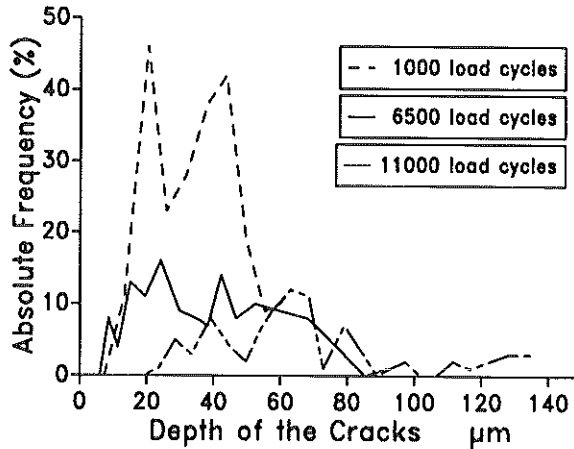
Fig 3 Histogram of the extension of the cracks in depth.
