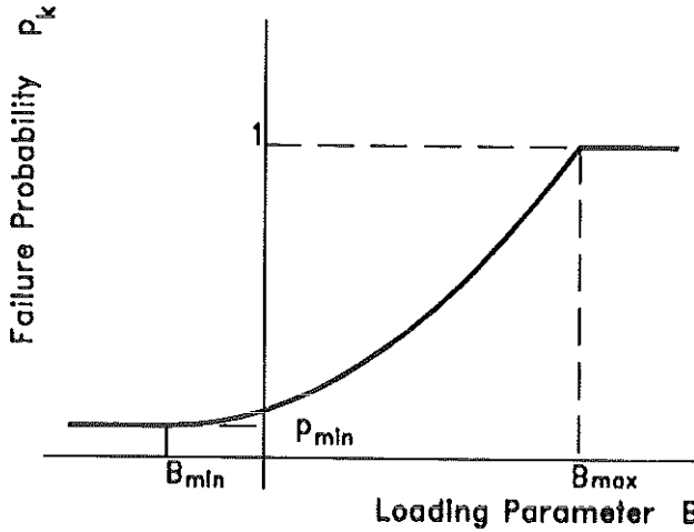
Fig 4 Relationship between the loading parameter and the failure probability.
