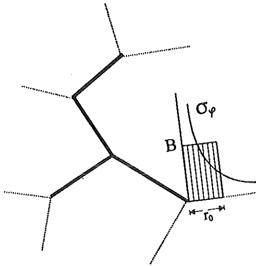
Fig 5 Normal stress distribution acting on the uncracked edges.
