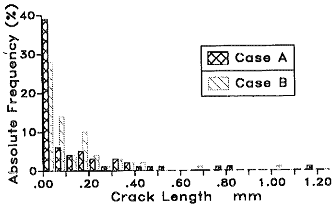
Fig 8 Crack length distribution of the simulated crack patterns.
