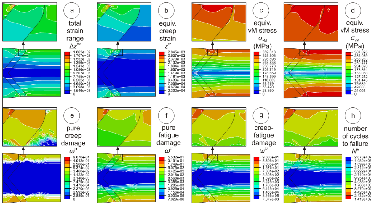
Figure 5. Contour plots of LMM results for type 1 weldment corresponding to \Delta \epsilon_{tot} = 1\% on the outer fiber of plate and \Delta t = 5 hours of dwell period
