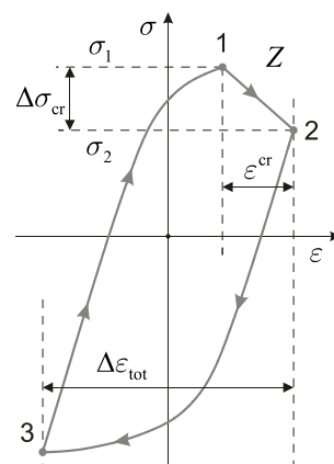
Figure 1. Typical saturated hysteresis loop with creep fatigue interaction
