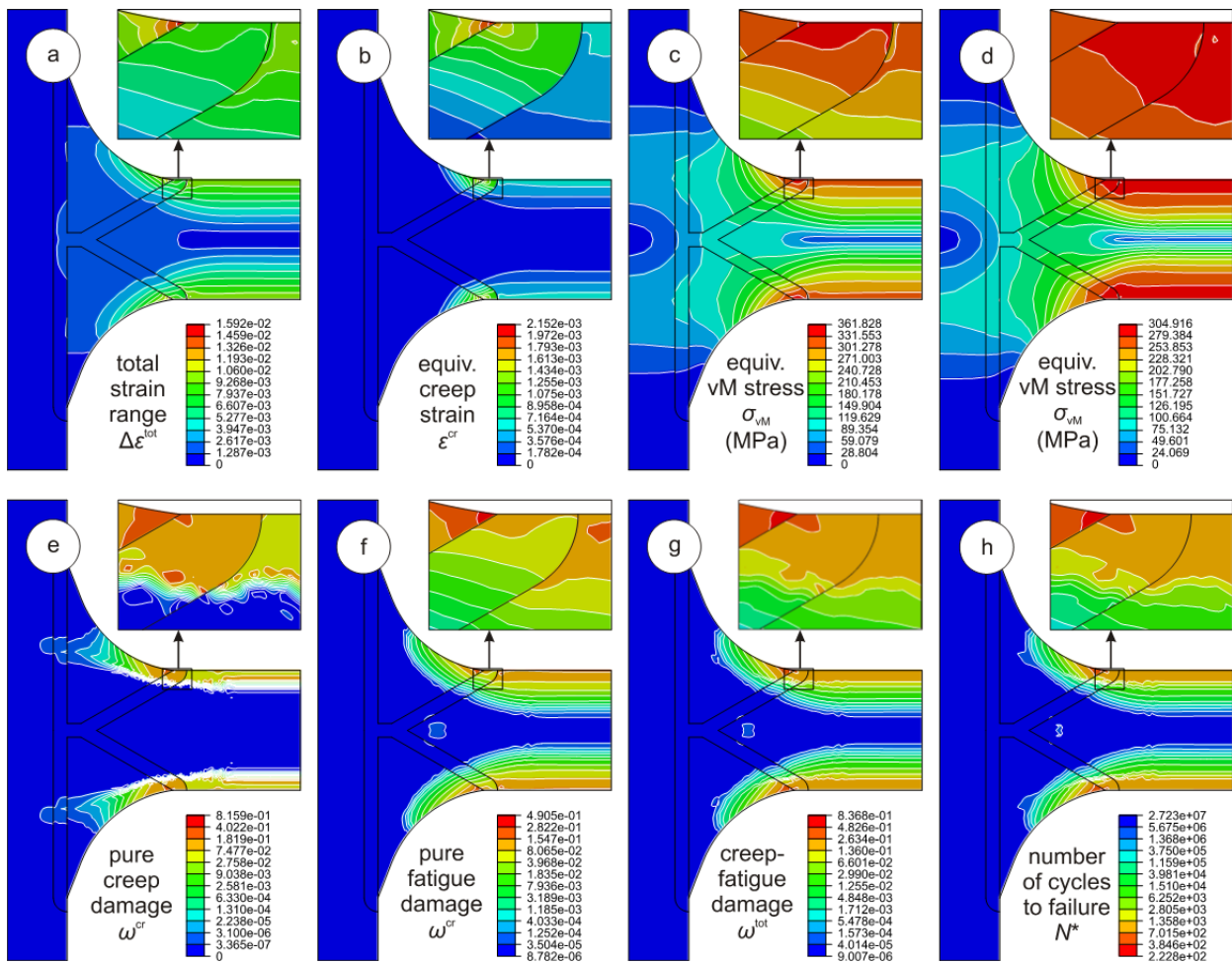
Figure 6. Contour plots of LMM results for type 2 weldment corresponding to \Delta \epsilon_{tot} = 1\% on the outer fiber of plate and \Delta t = 5 hours of dwell period
