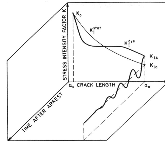
Fig. 8. Influence of dynamics effects on crack arrest.
