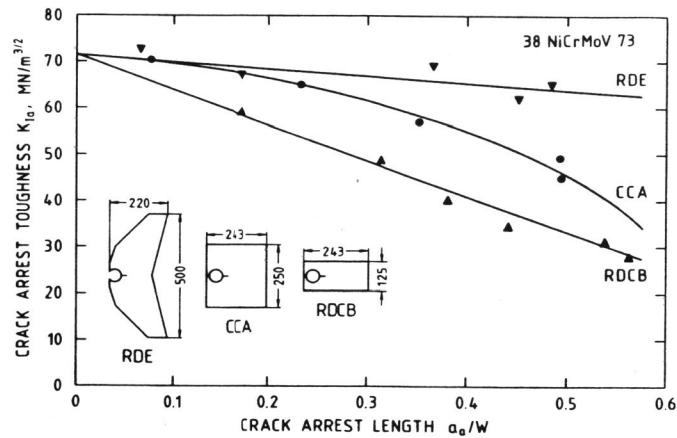
Fig. 7. Dependence of crack arrest fracture toughness on arrest crack length for different test specimens.
