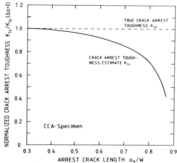
Fig. 9. Dynamic correction function.
