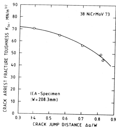
Fig. 5. Dependence of crack arrest fracture toughness K_{Ia} on crack jump distance for steel 38 NiCrMoV 73.
