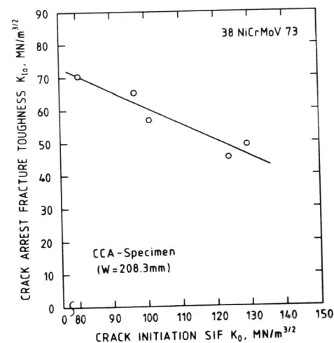
Fig. 6. Dependence of crack arrest fracture toughness K_{Ia} on crack initiation SIF for steel 38 NiCrMoV 73.
