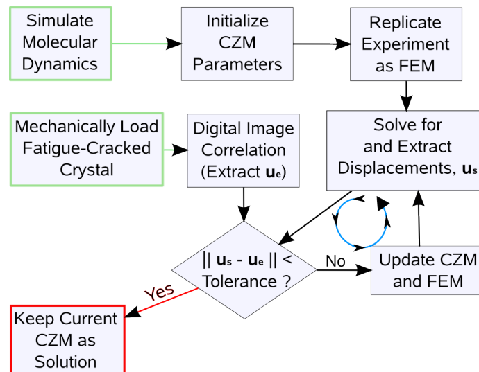
Fig. 3: Inverse approach to finding CZM parameters
