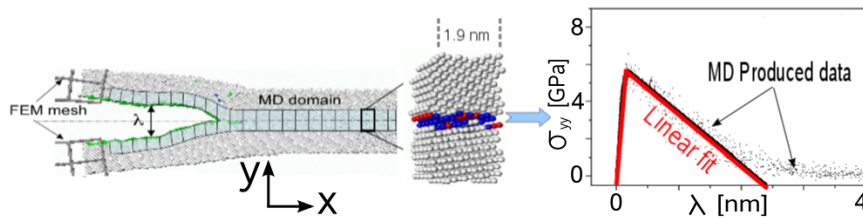
Fig. 1: CZM extraction from MD simulation [11]
