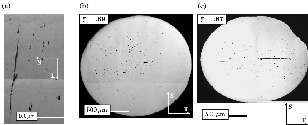
Figure 4: (a) Necklace coalescence under plane strain longitudinal loading. (b) & (c) Cross sections of round notched bars beneath fracture surface for two pipeline steels: (b) steel with no delamination; (c) steel with delamination. Loading is longitudinal in all.
