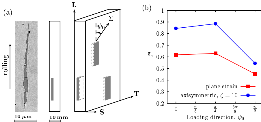
Figure 2: (a) MnS inclusion viewed in L-S and L-T planes. (b) Strain to failure versus loading orientation in L-T plane, \psi_0 .
