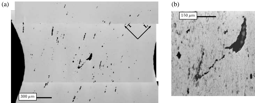
Figure 3: (a) Crack initiation in off-axes loading ( \psi_0 = 45^\circ ) due to (b) void-sheet coalescence.
