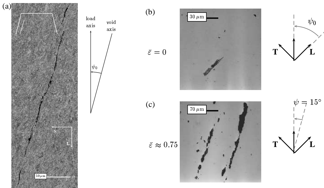
Figure 1: Void rotation (a) in longitudinal loading ( \psi_0 = 0^\circ ), (b) and (c) in off-axes loading ( \psi_0 = 45^\circ ). Sketch at the top in (a) indicates location of cavity near free surface of broken notched bar.
