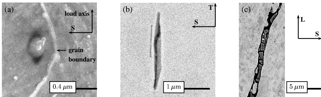
Figure 5: Void nucleation at small scale (a) by decohesion at the poles of a tiny MnS inclusion; (b) by inclusion fracture but no void growth ( \bar{\epsilon} \approx 0.3 ); note thinner unfractured inclusion. (c) Void nucleation at a larger inclusion by fragmentation then decohesion.
