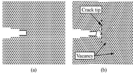
Figure 4: Atom configurations around the crack tip in specimen 1: (a) before cyclic loading; and (b) after the twelfth cycle.
