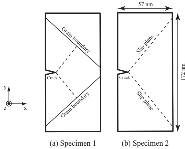
Figure 2: Schematic diagrams of specimens for a molecular dynamics simulation.
