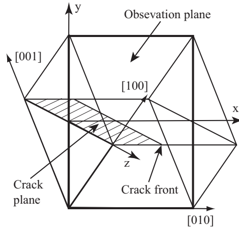
Figure 1: Relationship between a crystallographic orientation and a coordinate system of a crack.
