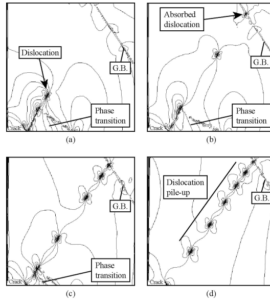
Figure 3: Time evolution of the distribution of the local stress \sigma_y between the crack tip and the grain boundary in specimen 1 during the first loading.
