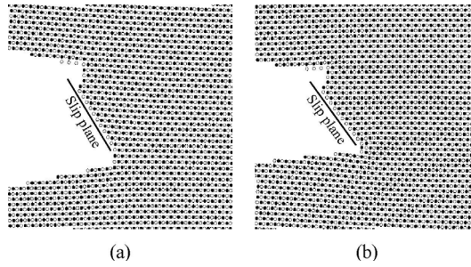
Figure 5: Atom configurations around the crack tip in specimen 2: (a) after the first loading; and (b) after the first unloading.
