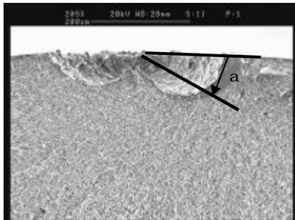
Fig.4 An interrupted crack found in a 12A100 nitrided and peened run-out specimen, \sigma_a=760 MPa.
