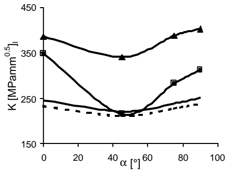
Fig.6 K values along the crack front: -? - specimen 12A100, broken, \sigma_a=780\text{MPa} ; -□- specimen 12A100, run-out, \sigma_a=760\text{MPa} ; —○— specimen N, broken, \sigma_a=380\text{MPa} ; ---○--- specimen N, run-out, \sigma_a=360\text{MPa} .
