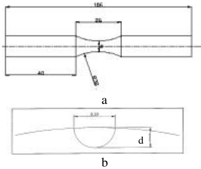
Fig.1 a) Specimen used for the rotating bending fatigue tests; b) particular of the micro-hole.
