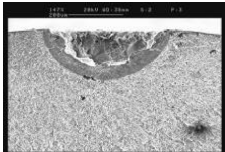
Fig.3 An arrested crack found in a nitrided run out specimen, \sigma_a=360 MPa.
