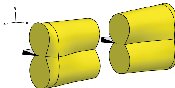
Figure 4: Calculated crack tip plastic zone along the crack front across the thickness of the specimen, schematically.
