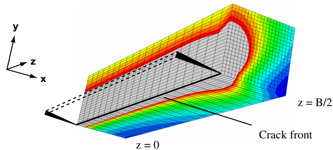
Figure 3: Three-dimensional view of the crack tip plastic zone ( B = 10 mm).
