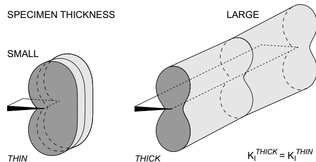
Figure 5: Simplified representation of the crack tip plastic zone along the crack front for specimens of small and large thickness.
