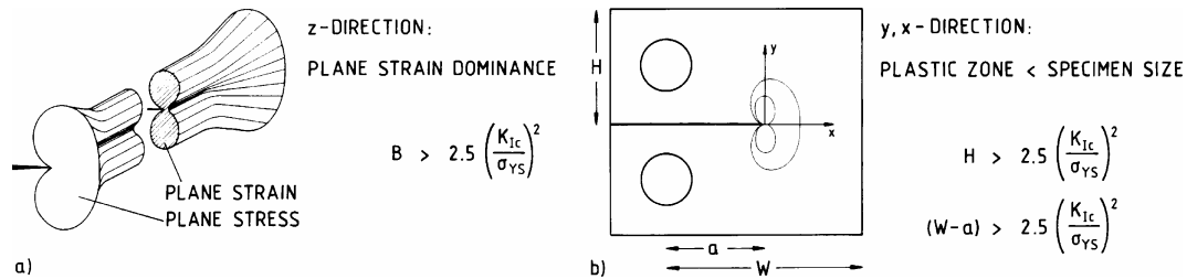
Figure 1: Validity criteria and “dog-bone” model with derived minimum size specimen requirements for determining the plane strain fracture toughness K_{Ic} .
