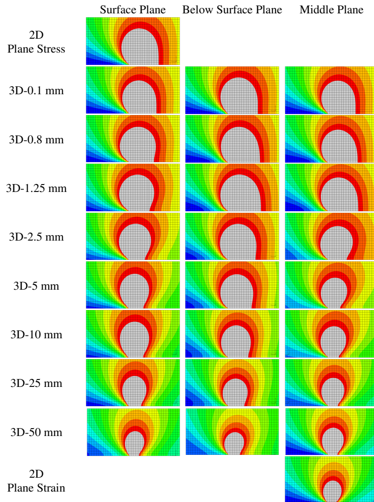
Figure 2: Crack tip plastic zones at the surface (left column), in a plane below the surface (middle column), and in the middle plane of the specimen (right column).
